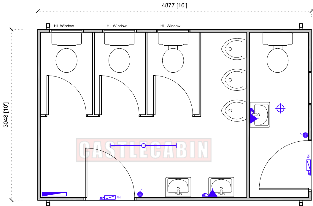
FLOOR PLAN SCALE 1:40
