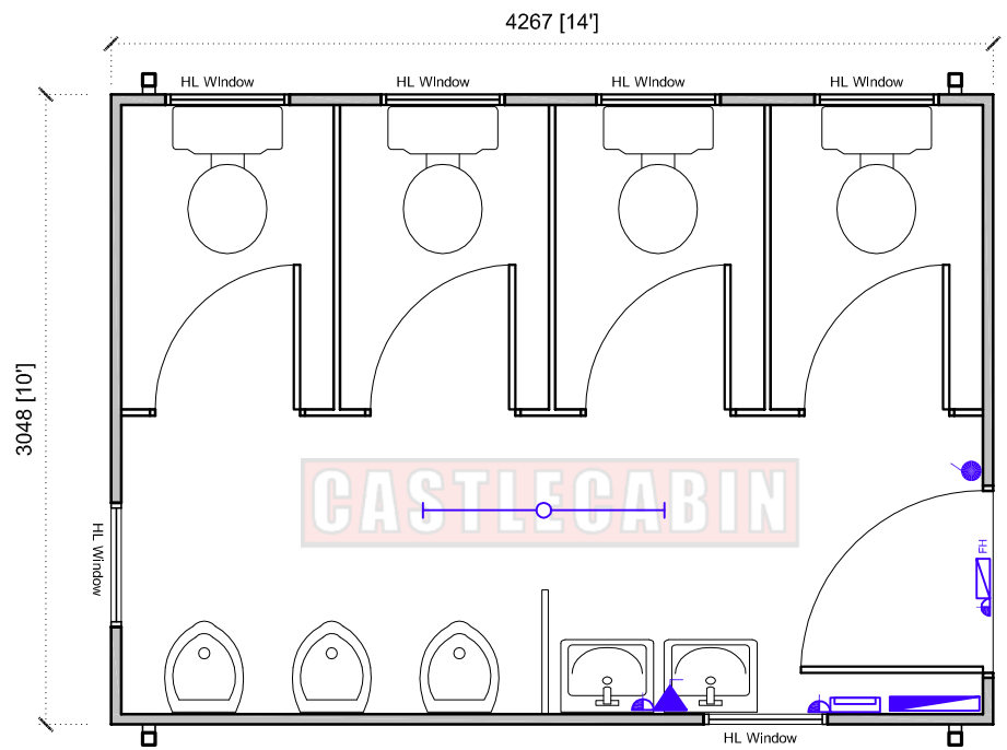
FLOOR PLAN SCALE 1:40
