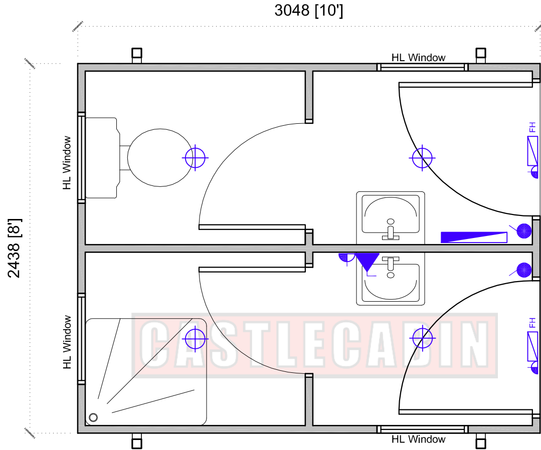
FLOOR PLAN SCALE 1:25
