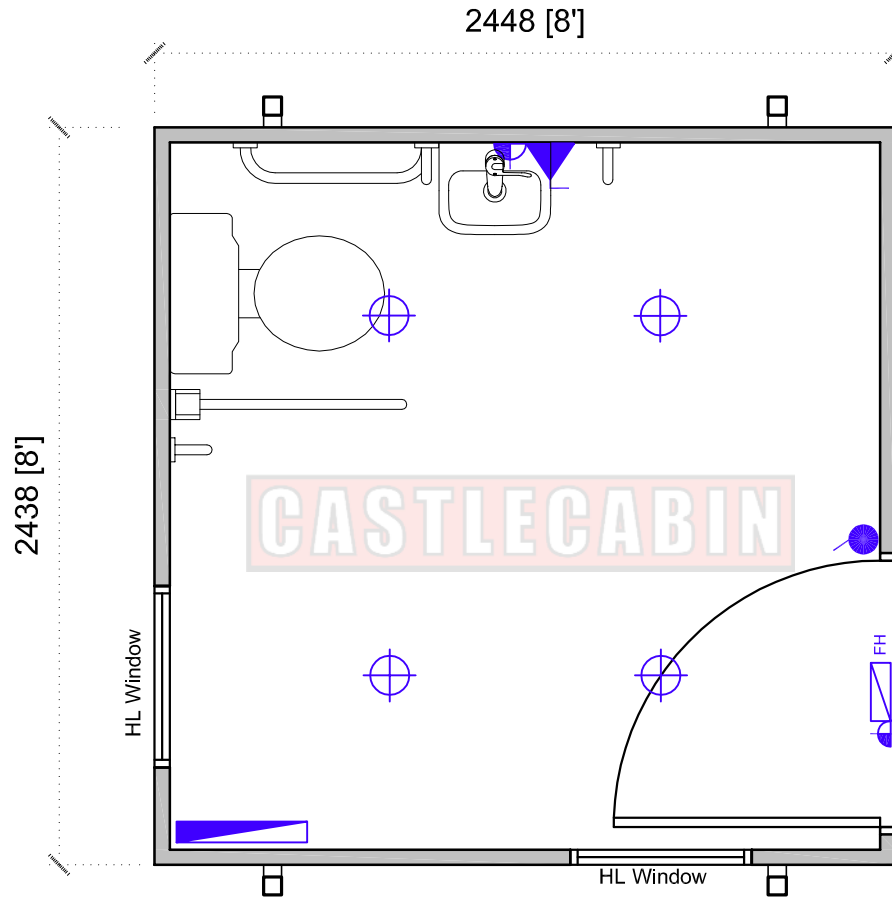
FLOOR PLAN SCALE 1:25
