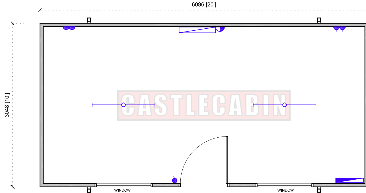
FLOOR PLAN SCALE 1:40
