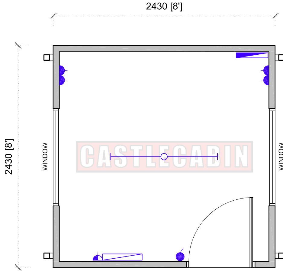
FLOOR PLAN SCALE 1:25
