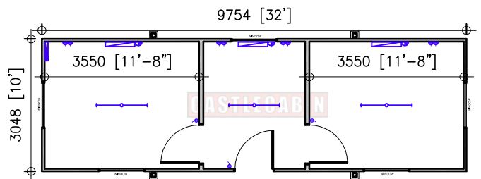
FLOOR PLAN
