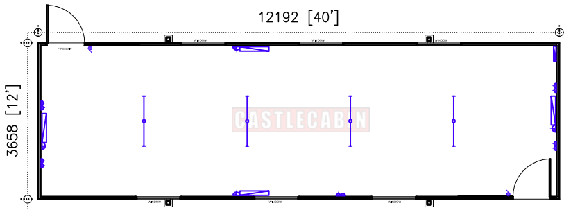
FLOOR PLAN
