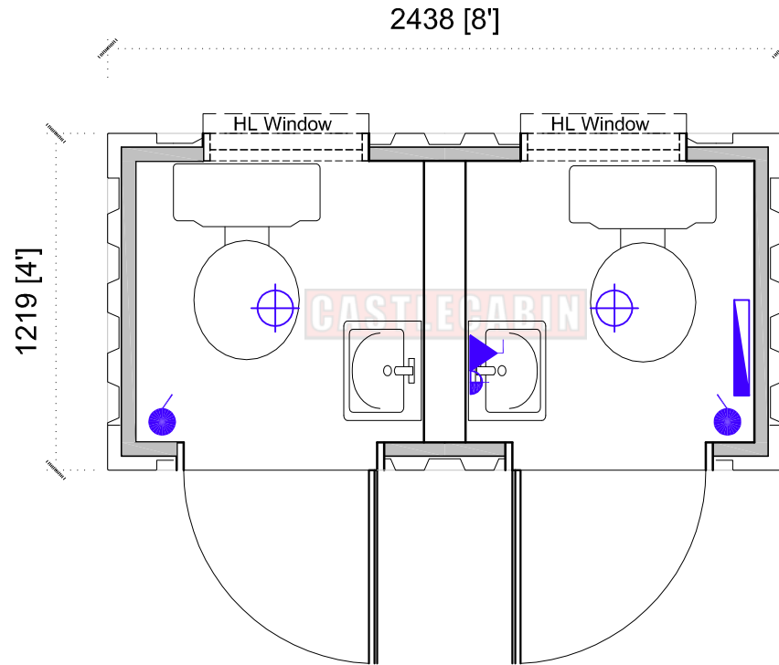
FLOOR PLAN SCALE 1:25
