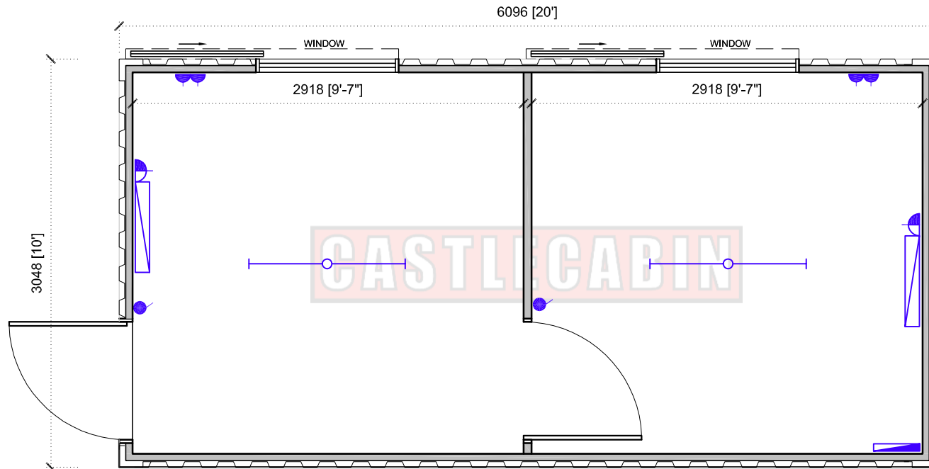
FLOOR PLAN SCALE 1:40
