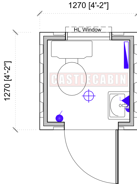
FLOOR PLAN SCALE 1:25
