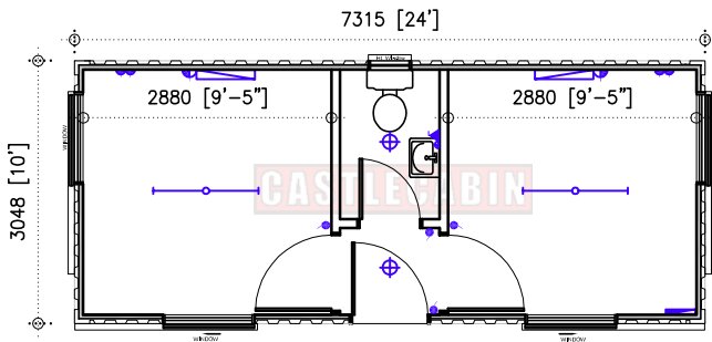
FLOOR PLAN
