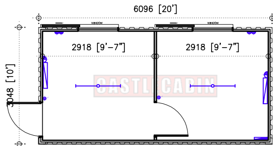
FLOOR PLAN
