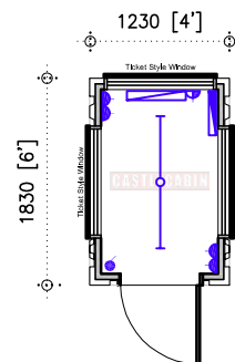
FLOOR PLAN
