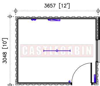
FLOOR PLAN
